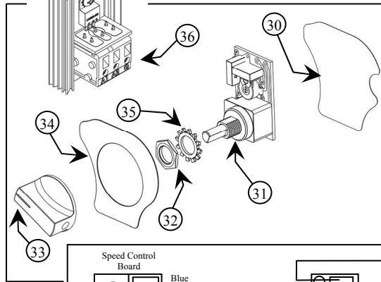
Variable Speed Diagram
